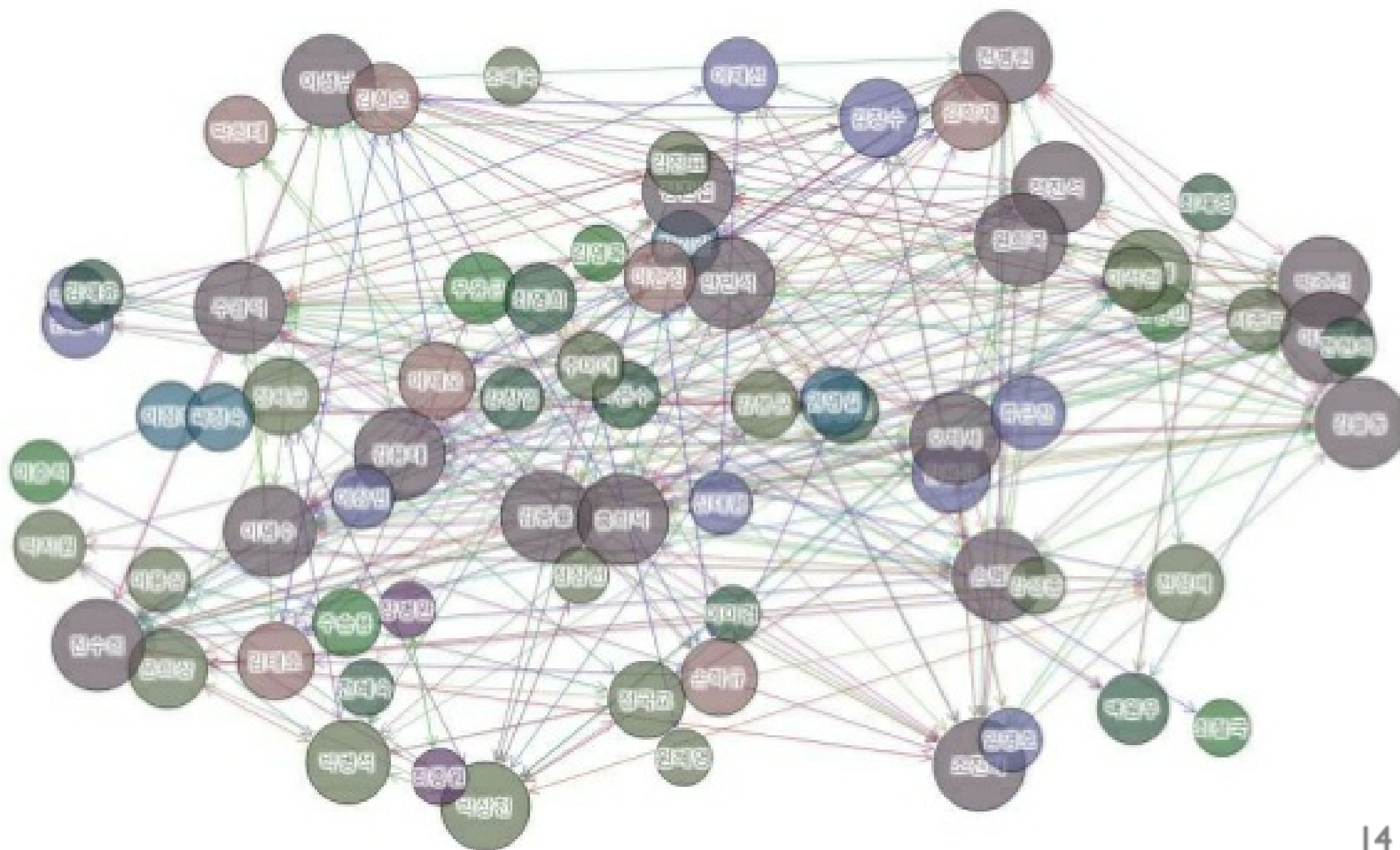
Network Graph
